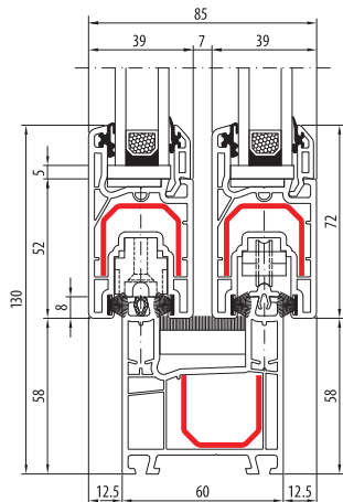
Duo Slide ST 60
